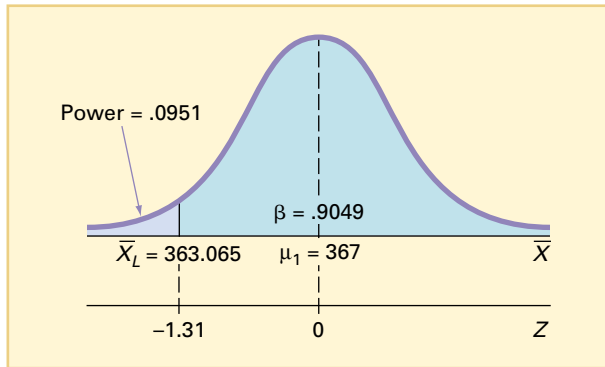
FIGURE 9.30 Determining the power of the test and the probability of a Type II error when \mu_1 = 367 grams
