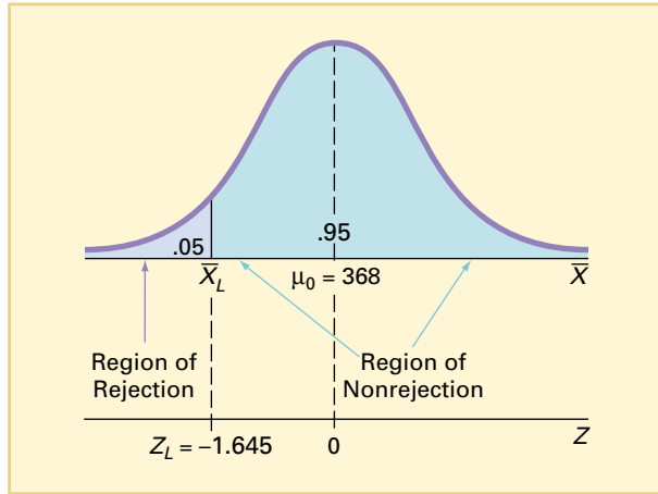
FIGURE 9.27 Determining the lower critical value for a one-tail Z test for a population mean at the 0.05 level of significance
