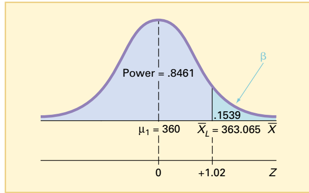
FIGURE 9.28 Determining the power of the test and the probability of a Type II error when \mu_1 = 360 grams
