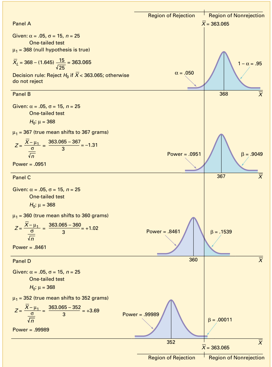
FIGURE 9.32 Determining statistical power for varying values of the actual population mean
