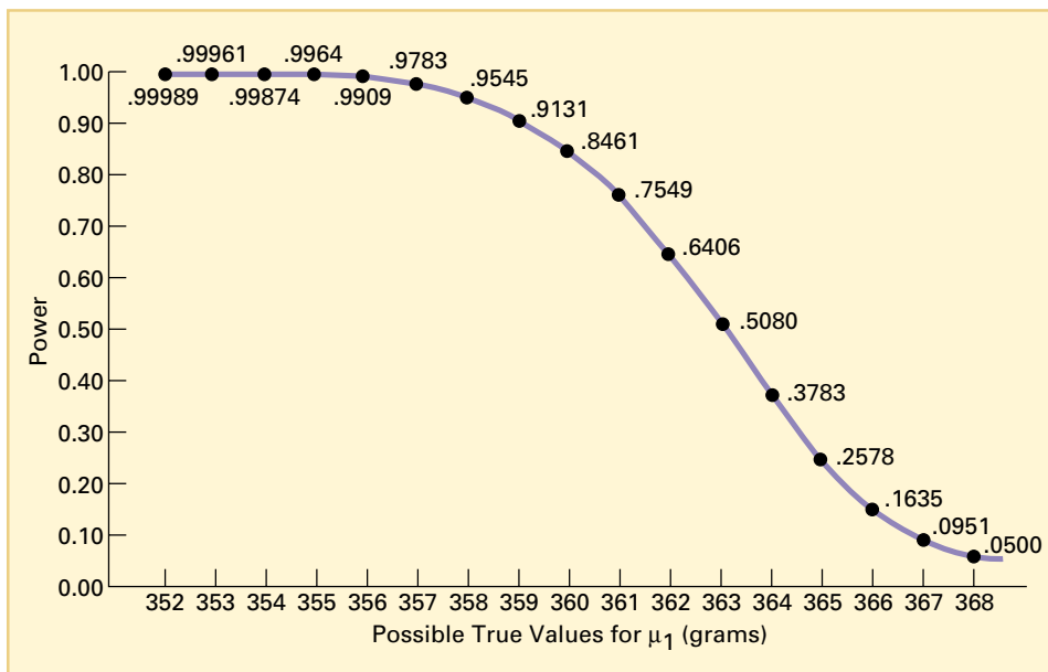
FIGURE 9.31 Power curve of the cereal-box-filling process for the alternative hypothesis H_1: \mu < 368 grams
