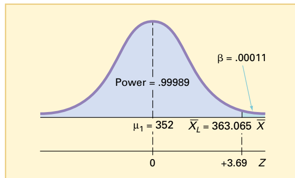
FIGURE 9.29 Determining the power of the test and the probability of a Type II error when \mu_1 = 352 grams
