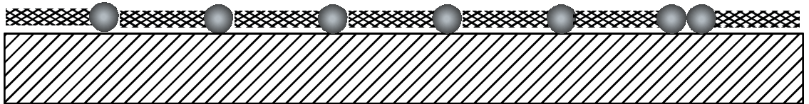
(c) Saturated surface aligned phase
