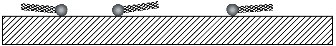
(a) Disordered, mobile lattice gas
