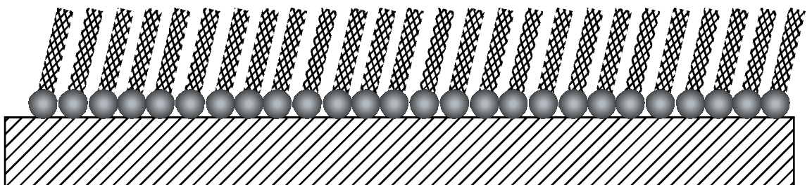
(e) Saturated solid phase
