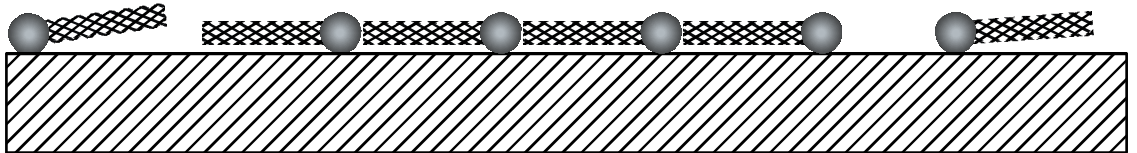
(b) Lattice gas + ordered islands
