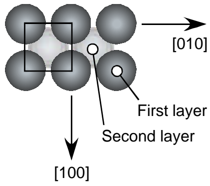
(a) bcc(100)
