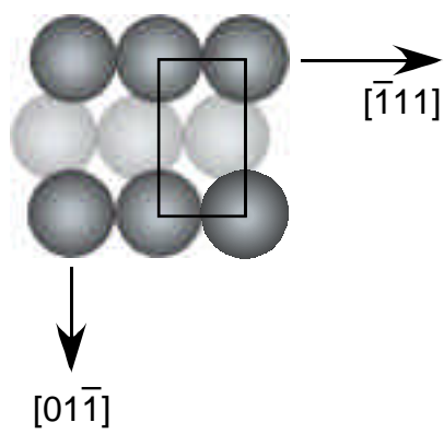
(c) bcc(211)
