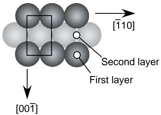
(c) fcc(110)
