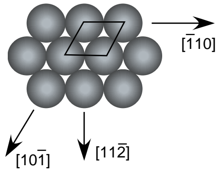
(b) fcc(111)
