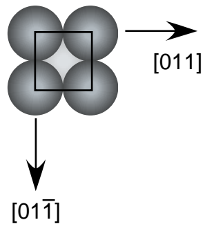
(a) fcc(100)
